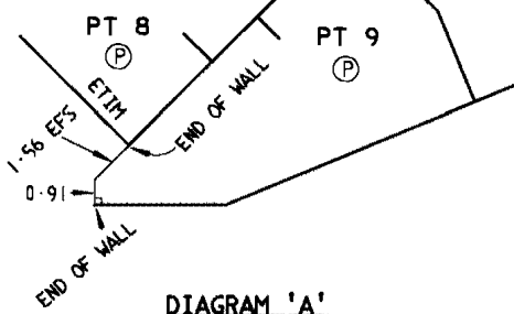
DIAGRAM 'A' RR 1:200
