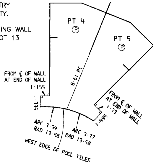
DIAGRAM 'B' RR 1:200
